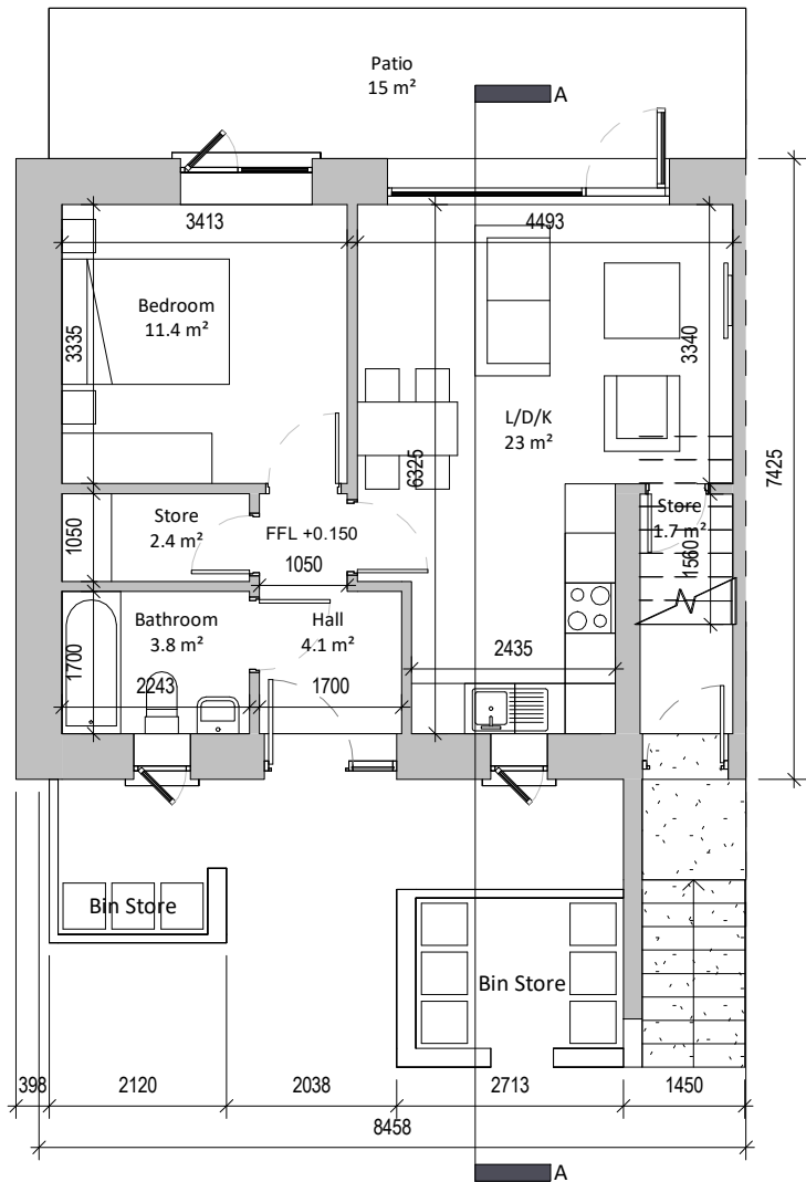
① Ground Floor (Simplex 1LA) 1 : 100
