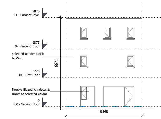
2 Rear Elevation 1 : 200
