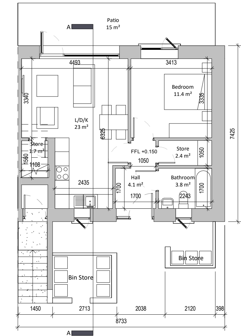
① Ground Floor (Simplex 1RA) 1 : 100
