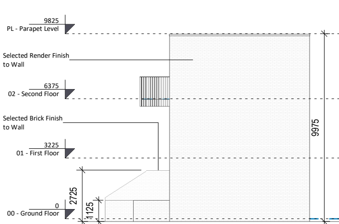
3 Side Elevation (Right) 1 : 200
