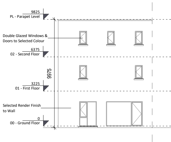
2 Rear Elevation 1 : 200
