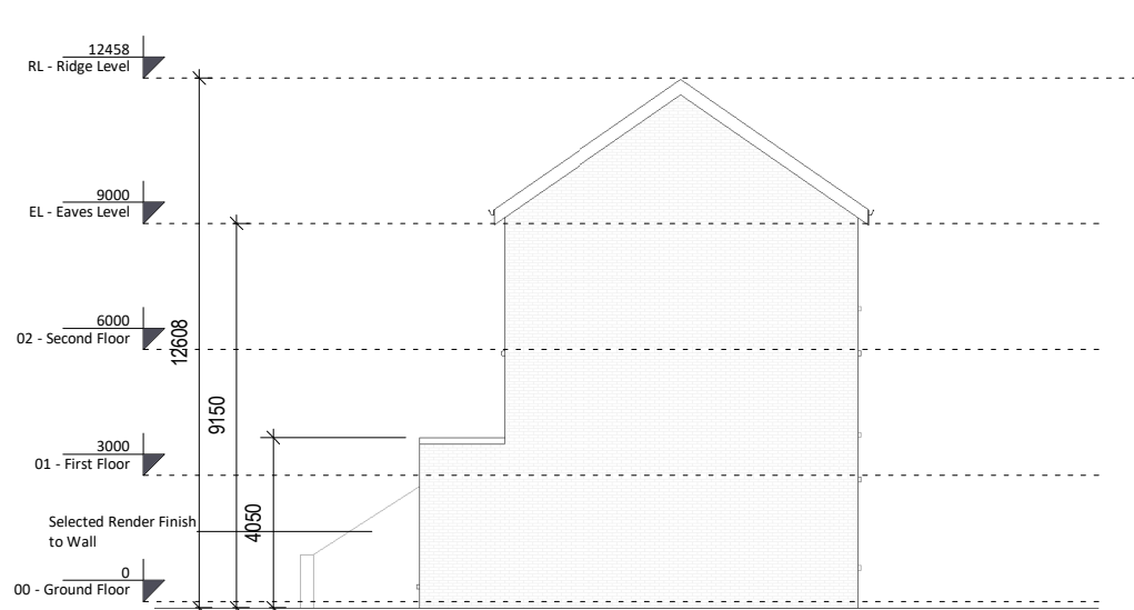
3 Side Elevation (Right) 1 : 200
