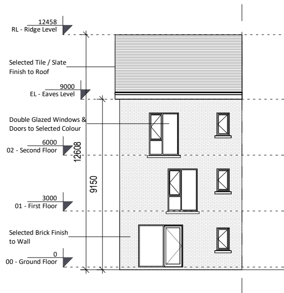
2 Rear Elevation 1 : 200
