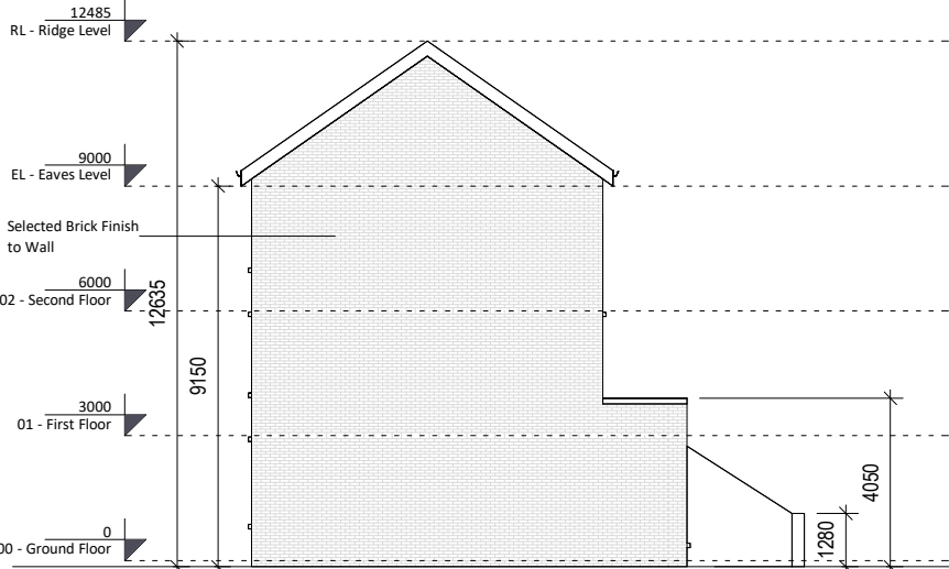
3 Side Elevation (Left) 1 : 200
