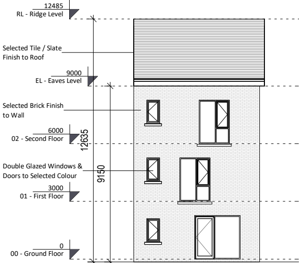
2 Rear Elevation 1 : 200
