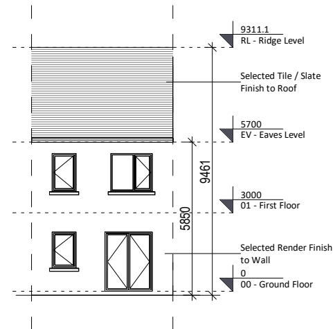
4 Rear Elevation 1 : 200
