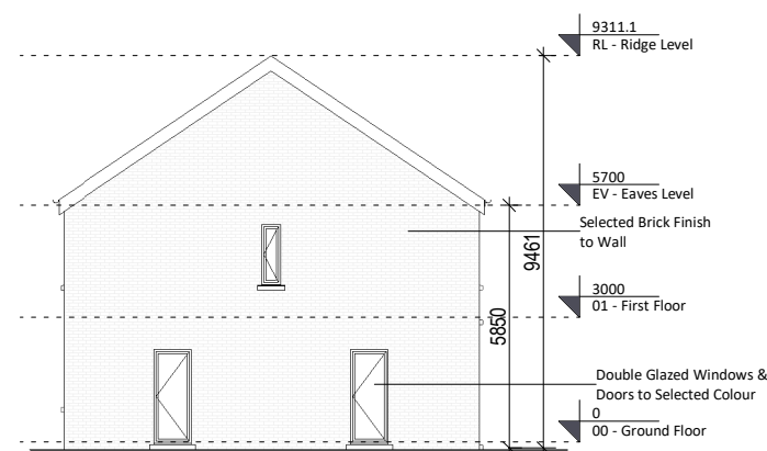
5 Side Elevation 1 : 200
