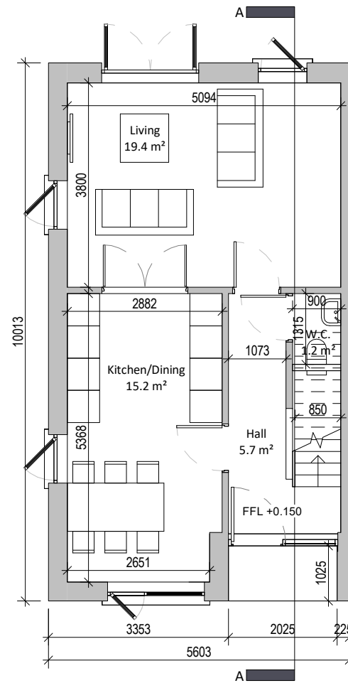
1 Ground Floor 1 : 100
