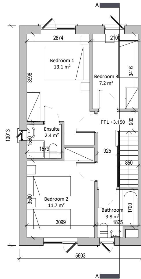
2 First Floor 1 : 100
