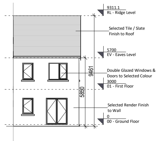
4 Rear Elevation 1 : 200
