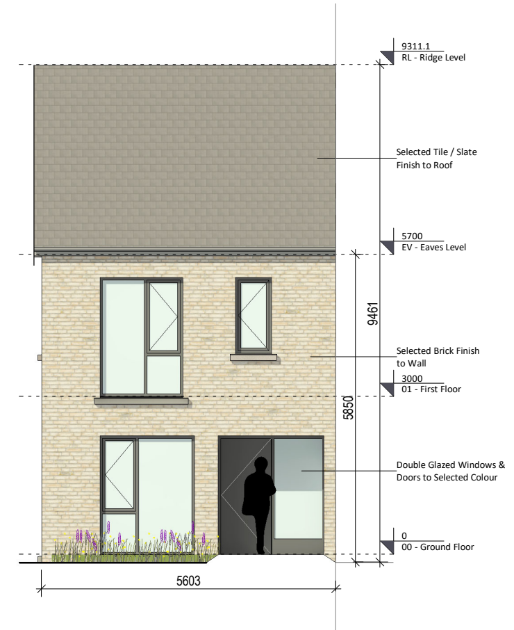
3 Front Elevation 1 : 100
