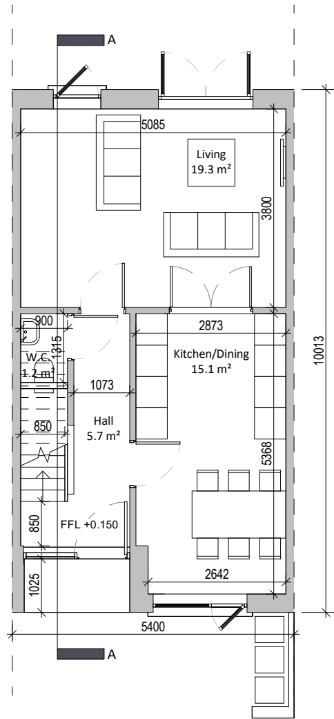
1 Ground Floor 1 : 100
