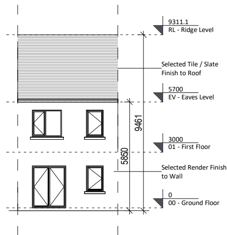
4 Rear Elevation 1 : 200
