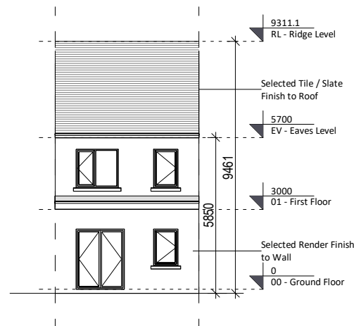
4 Rear Elevation 1 : 200
