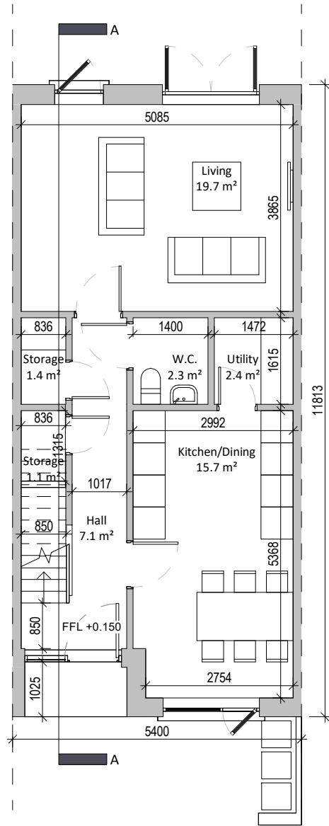
1 Ground Floor 1 : 100
