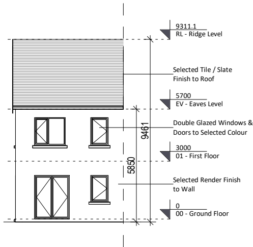
4 Rear Elevation 1 : 200
