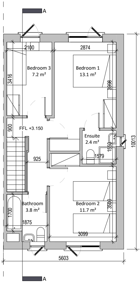
2 First Floor 1 : 100
