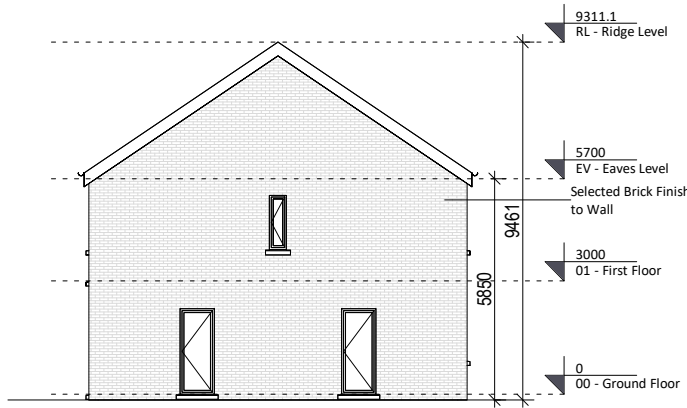
5 Side Elevation 1 : 200
