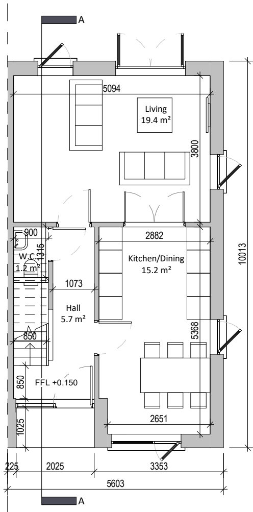
1 Ground Floor 1 : 100
