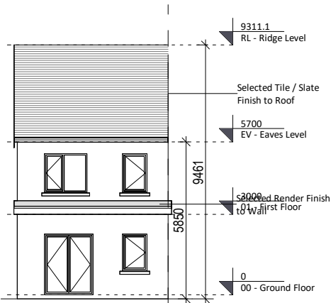
④ Rear Elevation 1 : 200
