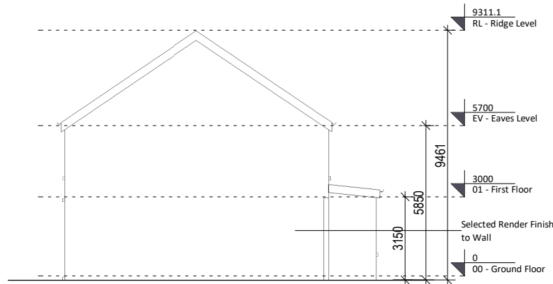
⑤ Side Elevation 1 : 200
