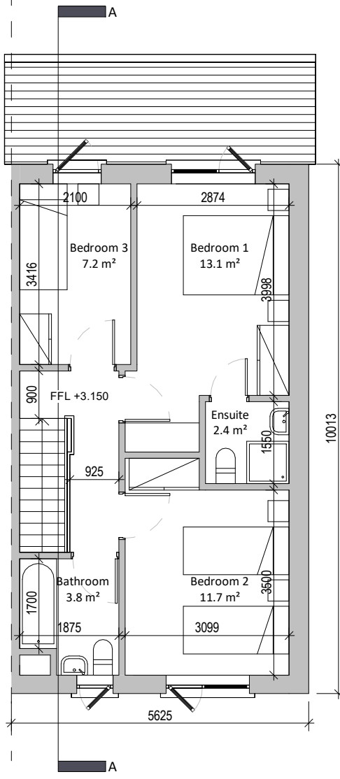
② First Floor 1 : 100
