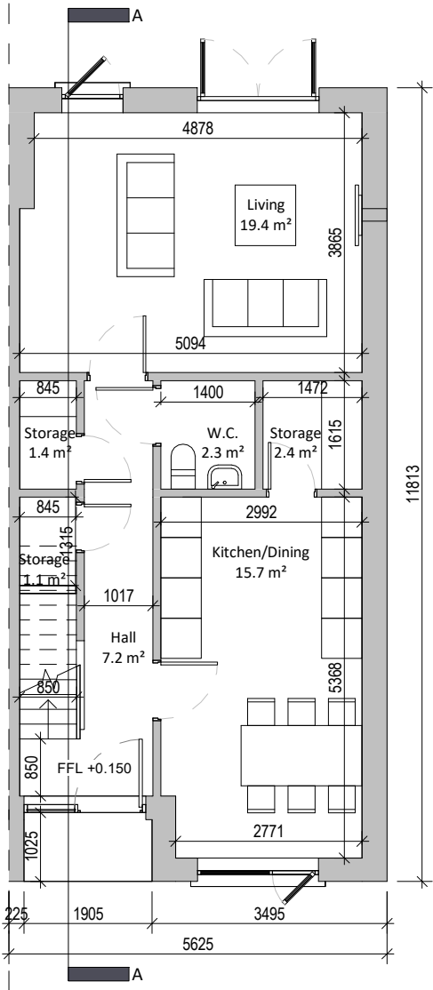
① Ground Floor 1 : 100
