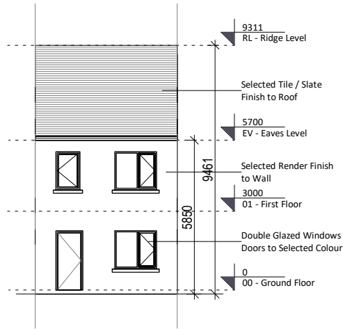
4 Rear Elevation 1 : 200
