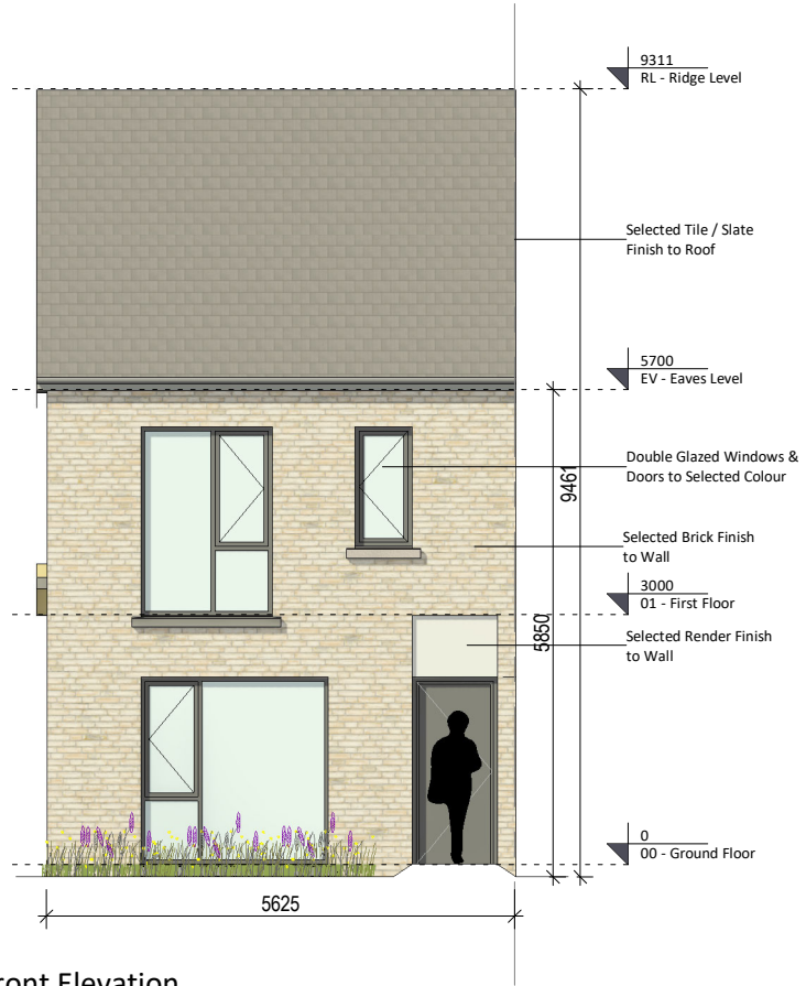
③ Front Elevation 1 : 100
