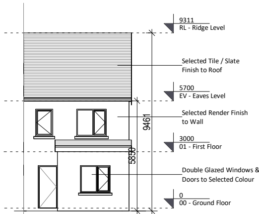
④ Rear Elevation 1 : 200
