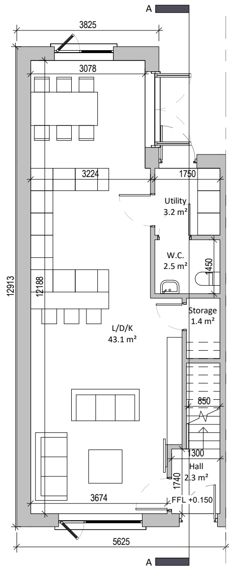
① Ground Floor 1 : 100
