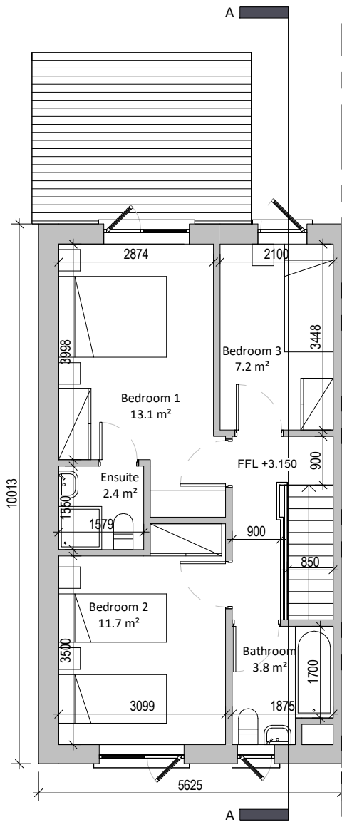
② First Floor 1 : 100
