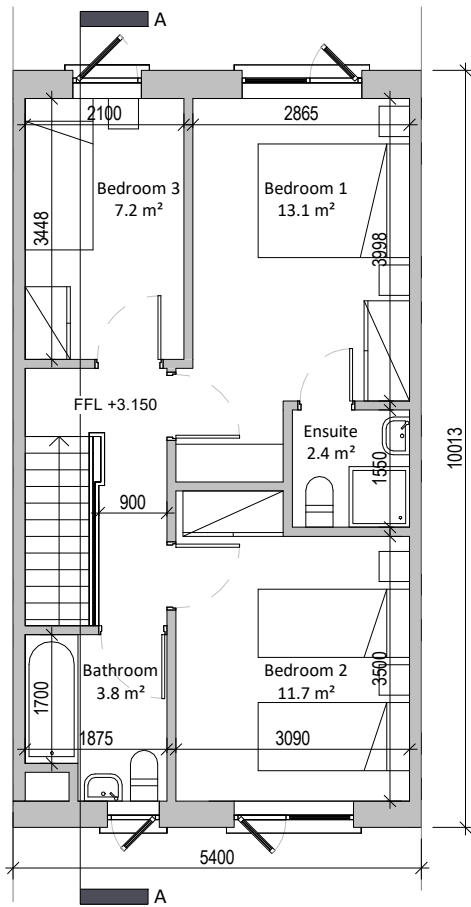
2 First Floor 1 : 100
