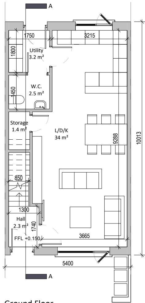
1 Ground Floor 1 : 100
