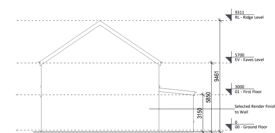
⑤ Side Elevation 1 : 200
