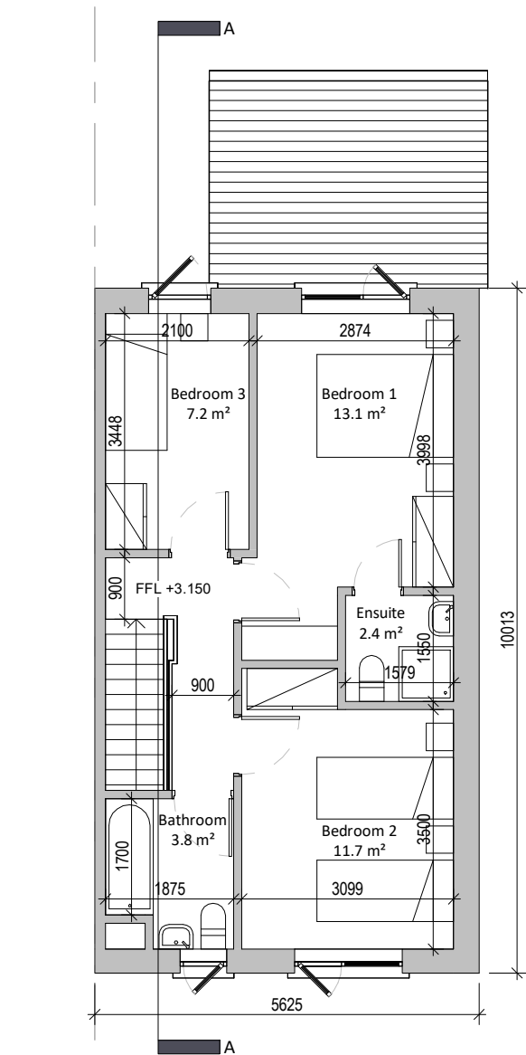
② First Floor 1 : 100
