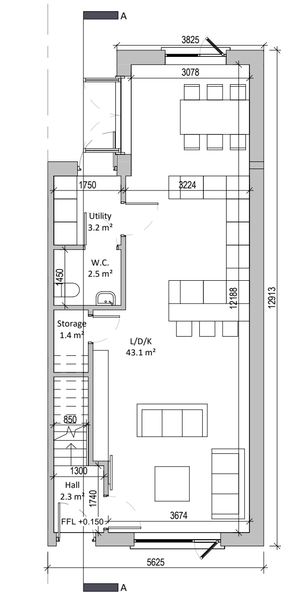
① Ground Floor 1 : 100
