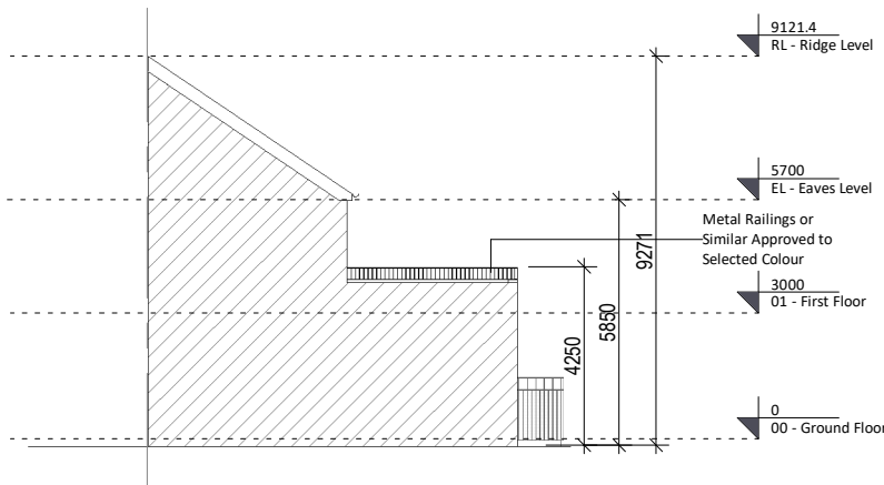
④ Side Elevation (Left) 1 : 200
