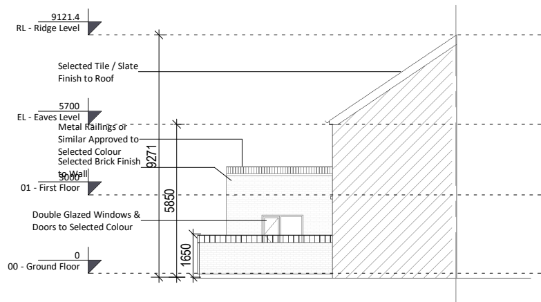
⑤ Side Elevation (Right) 1 : 200
