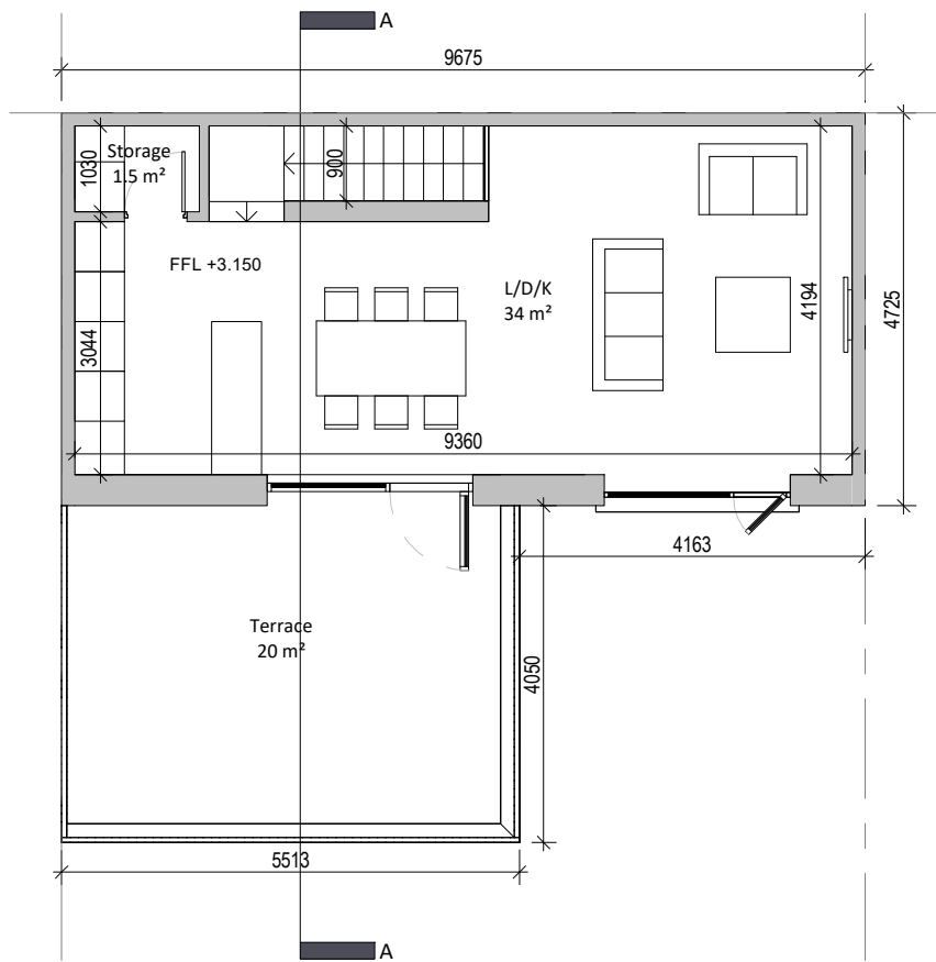
② First Floor 1 : 100
