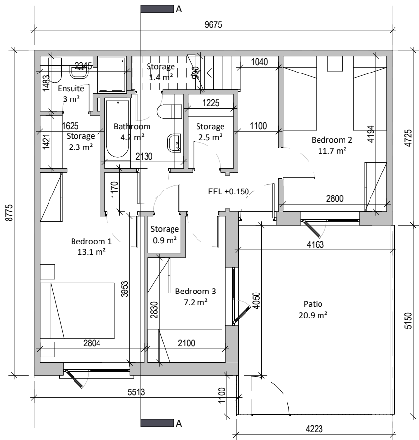
① Ground Floor 1 : 100
