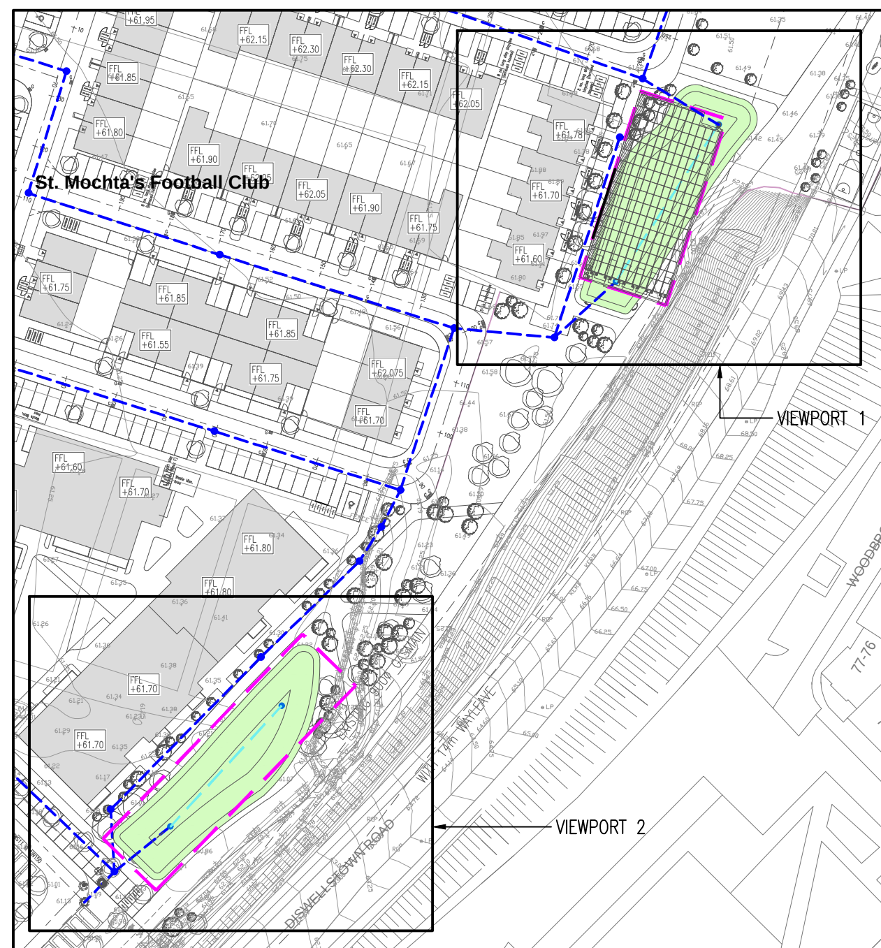
KEYPLAN SCALE 1:1000
