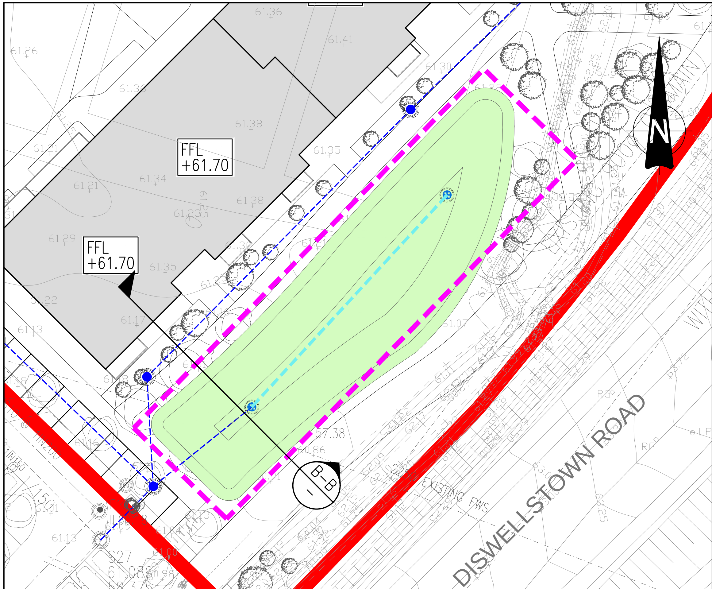
PLAN – ATTENUATION BASIN 2 (VIEWPORT 2) SCALE 1:250
